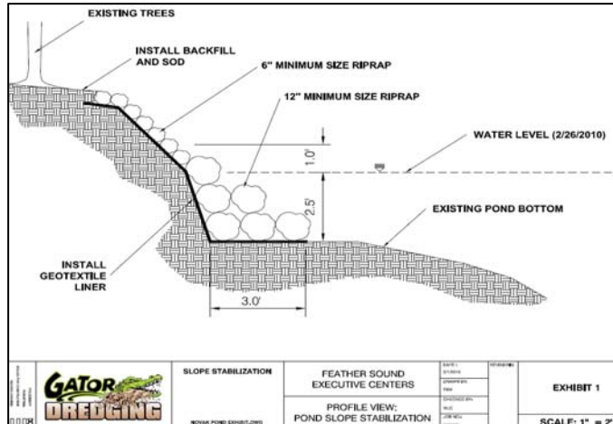
Proposed Bank Section View
